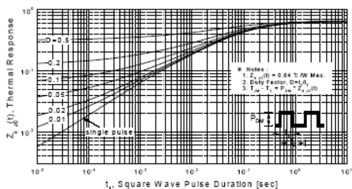
Figure 11-1. Transient Thermal Response Curve for HM13N50
