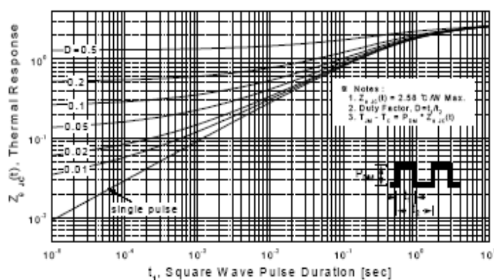
Figure 11-2. Transient Thermal Response Curve for HM13N50D
