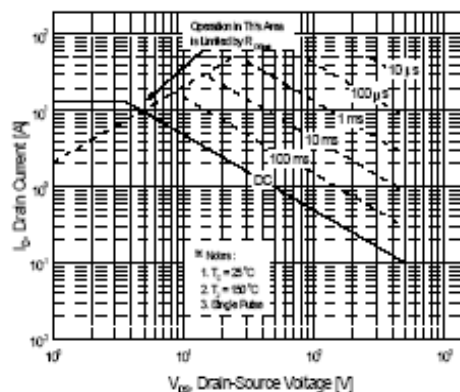
Figure 9-2. Maximum Safe Operating Area for HM13N50D
