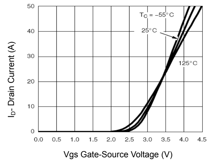
Figure 7 Transfer Characteristics
