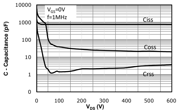
Fig 11: Capacitance Characteristics
