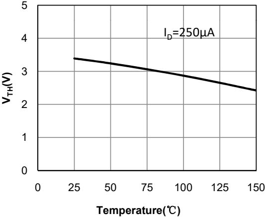
Fig 4: V_{TH} vs. T_J Temperature Characteristics
