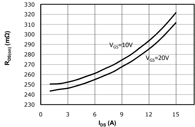
Fig 5: R_{DS(on)} vs. I_{DS} Characteristics ( T_J=25^{\circ}\text{C} )
